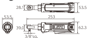
H-shaped head
