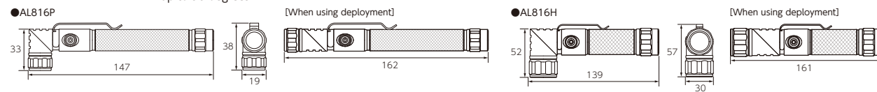
The head part can be rotated steplessly up to 90 degrees.
