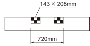
MAGNET TARGET SHEET (DAIHATSU1) No.AT120-031
