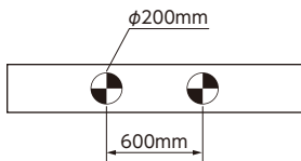
MAGNET TARGET SHEET (NISSAN1) No.AT120-041
