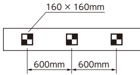
MAGNET TARGET SHEET (TOYOTA1) No.AT120-011
