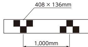
MAGNET TARGET SHEET (MAZDA2) No.AT120-082
