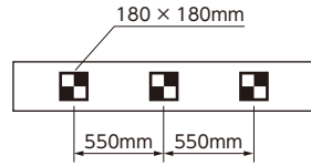
MAGNET TARGET SHEET (TOYOTA2) No.AT120-012
