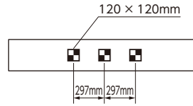
MAGNET TARGET SHEET (TOYOTA3) No.AT120-013
